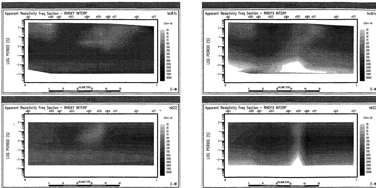
Fig. 15. Comparison of field and model apparent resistivity data for the model illustrated in Fig. 14. The top two pseudosections are the field data, whereas the bottom two are the modelled ones. The left column gives the E-polarization responses, whereas the right column gives the B-polarization ones.
