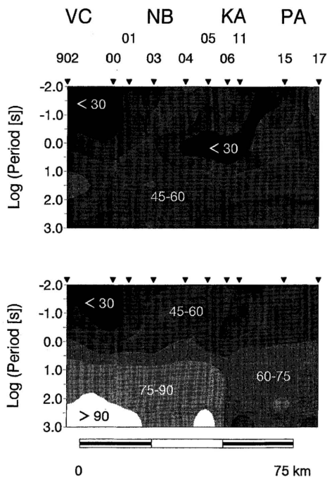
Fig. 11. Phase pseudosections of the decomposed \phi_{xy} (top) and \phi_{yx} (bottom) phases in strike co-ordinate system, with x pointing at -30^\circ , for a reduced set of responses. The contour interval is 15^\circ ; black regions denote phases below 30^\circ , whereas white regions denote phases greater than 90^\circ .
