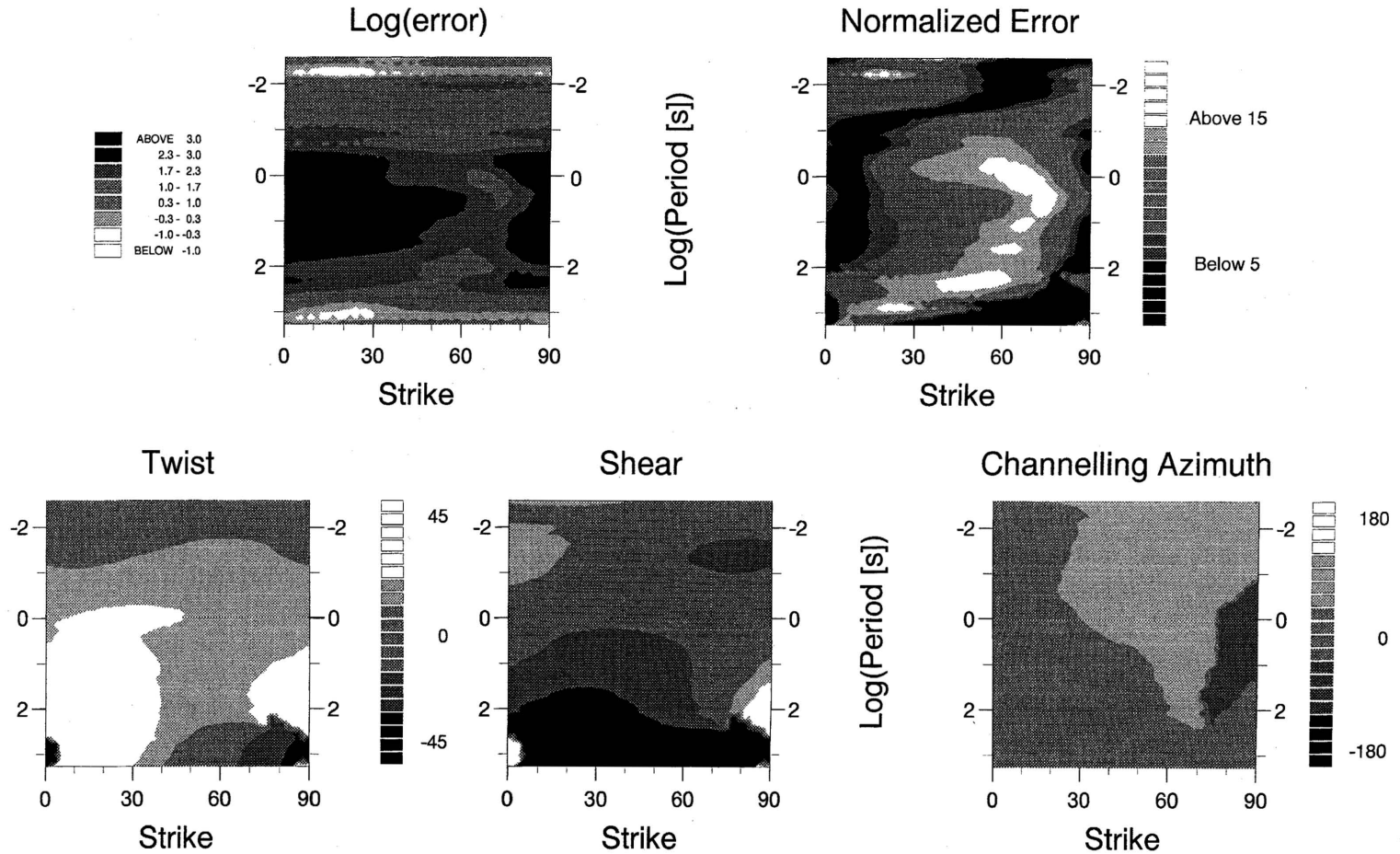
Fig. 3. (b) Grey-scale contour plots of the variation of the decomposition parameters with strike direction from 0^\circ to 90^\circ . The normalized error is a normalized, non-linear, inverted scale (see GKJB); values in excess of 15 ( white ) show strikes which are best-fitting, whereas values less than 5 ( black ) show the worst-fitting strikes.
