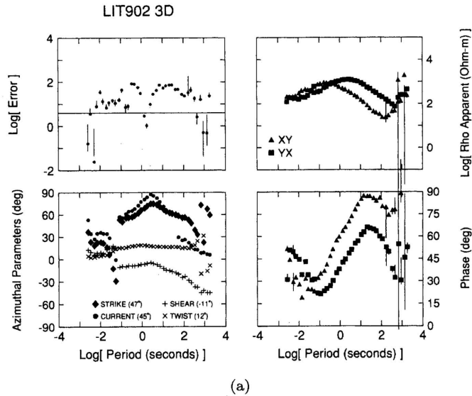
Fig. 3. (a) The unconstrained GB parameters for a 3D/2D model for the data from site lit902 . All diagrams are as for Fig. 2, with the exception of; Lower left GB distortion parameters strike ( diamonds ), shear ( pluses ), twist ( crosses ) and local current channelling ( circles ). The values in brackets after each parameter is the average value over the whole period range.
