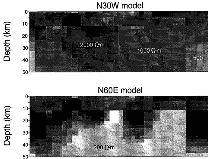
Fig. 18. The two 2D models found using Occam2 inversion with a vertical exaggeration of 1:1 (see text for details); top model fits high frequency data (>1 Hz) and E-polarization data in the range 10–100 s; bottom model fits high frequency data (>1 Hz) and B-polarization data in the range 10–100 s. Contour interval is 1/3 of a decade, from 100 \Omega\cdot\text{m} (white) to 5,000 \Omega\cdot\text{m} (black).
