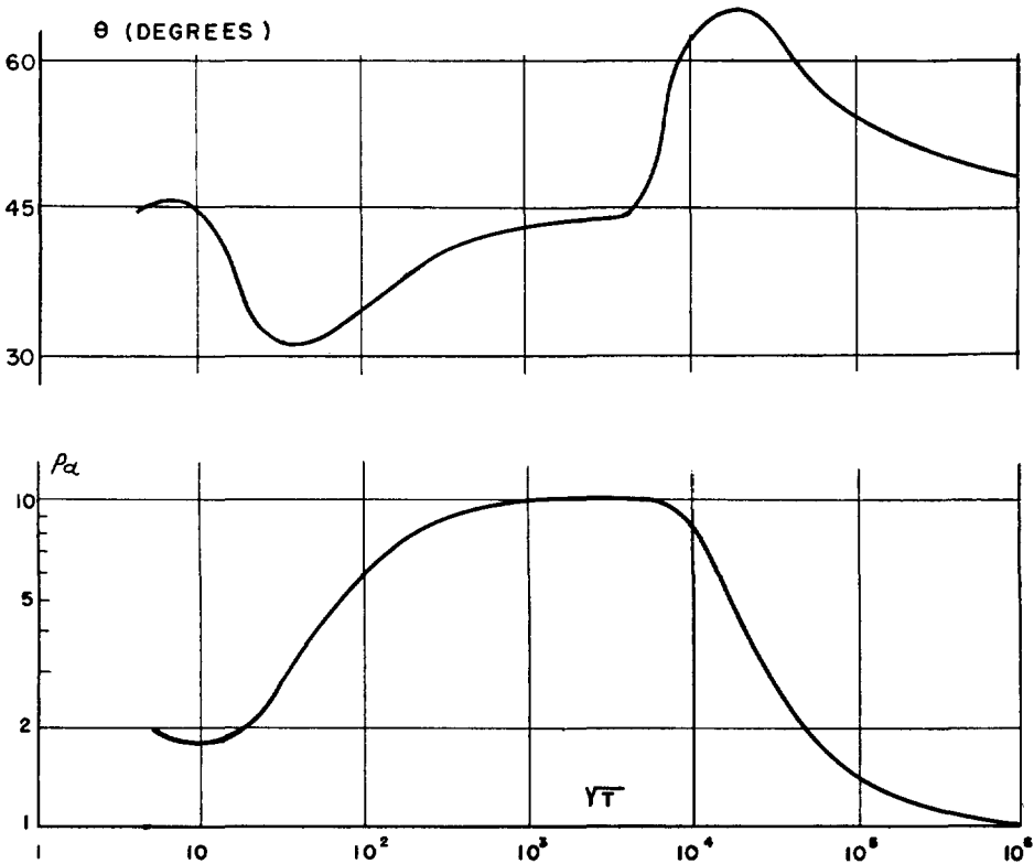
FIG. 9. Computed curves for hypothetical magneto-telluric sounding over three layers in which thickness of second layer is 900 times that of first and in which \rho_1, \rho_2 , and \rho_3 are in the ratio of 2:10:1.
