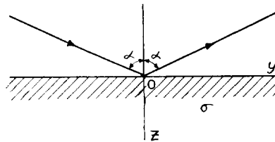
FIG. 4. Plane electromagnetic wave incident upon earth's surface.
