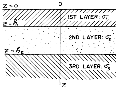
FIG. 6. Three-layer earth section.
