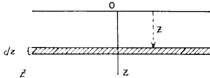
FIG. 3. Section showing horizontal uniform sheet of current.
